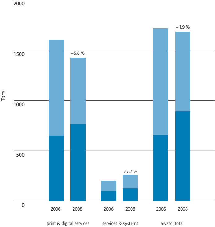
Acidification potential in SO 2 equivalents
