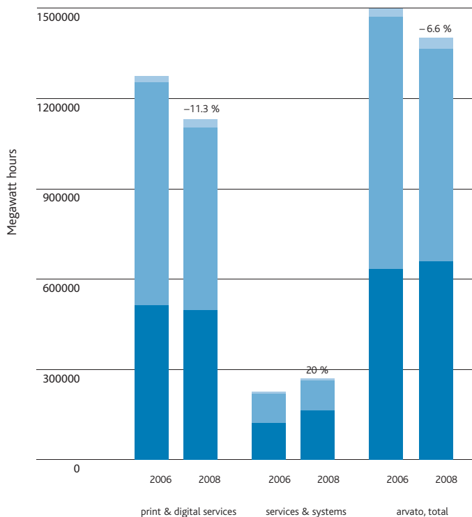
Energy usage in megawatt hours
