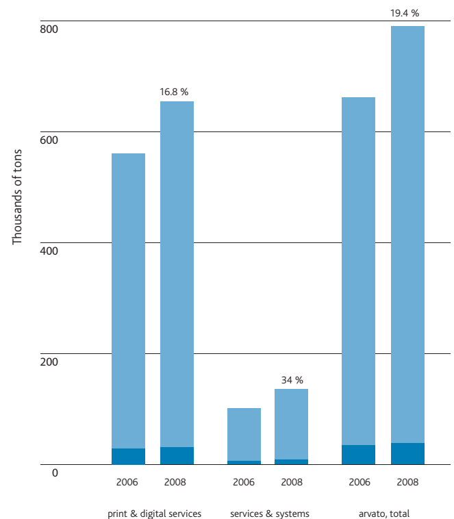
Greenhouse effect in CO 2 equivalents
