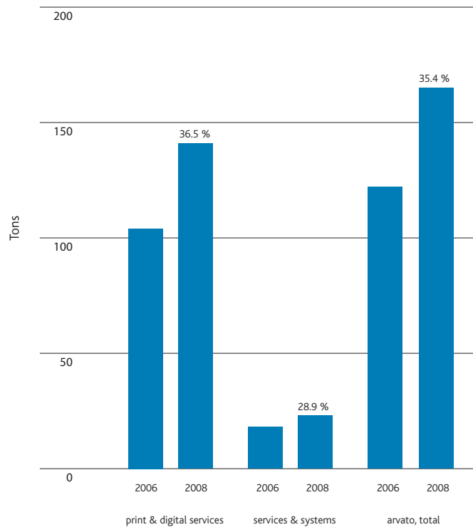
Eutrophication potential in PO 4 equivalents
