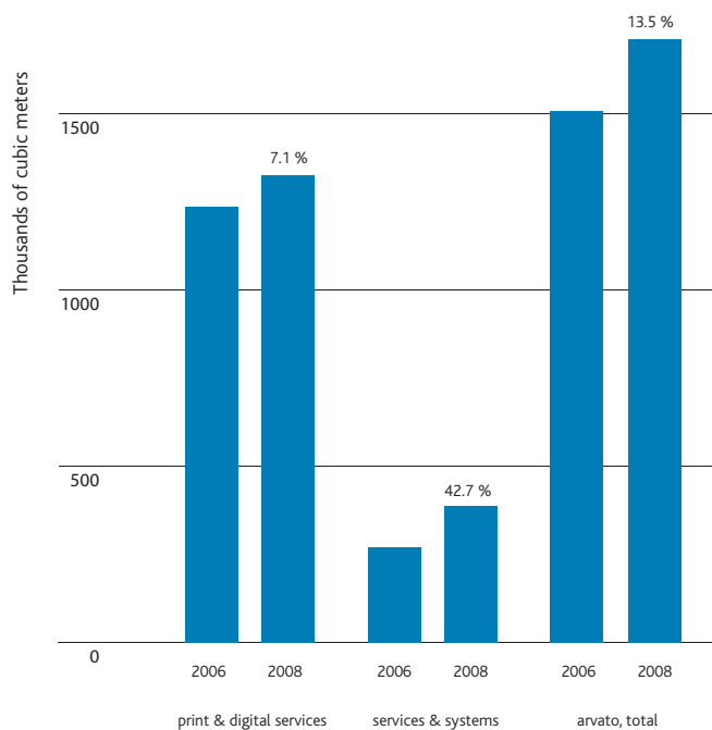
Water usage in cubic meters
