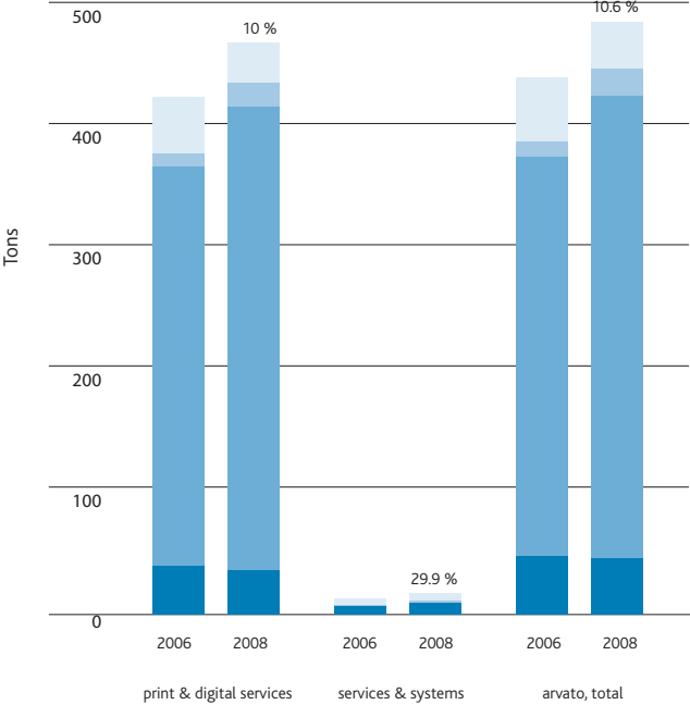
Summer smog potential in ethene equivalents
